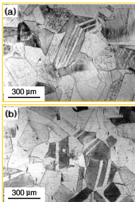
Fig. 6. Optical micrographs of (a) type 316LN SS with 0.002 wt.% N, and (b) 20 wt.% Mn-substituted type 316LN SS with 0.314 wt.% N. Chemical etching with a solution of 10% HCl + 10% \text{HNO}_3 + 15% acetic acid + 65% distilled water
