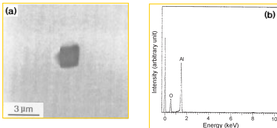
Fig. 8. (a) SEM image and (b) TEM/EDX spectrum of an alumina inclusion, which is commonly found in 20 wt.% Mn-substituted type 316LN SS with 0.317 wt.% N
