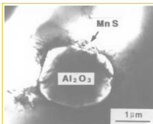
Fig. 9. TEM bright field image of MnS attached to Al 2 O 3 , showing that MnS had nucleated and grown on Al 2 O 3 , taken from 20 wt.% Mn-substituted type 316LN SS with 0.317 wt.% N
